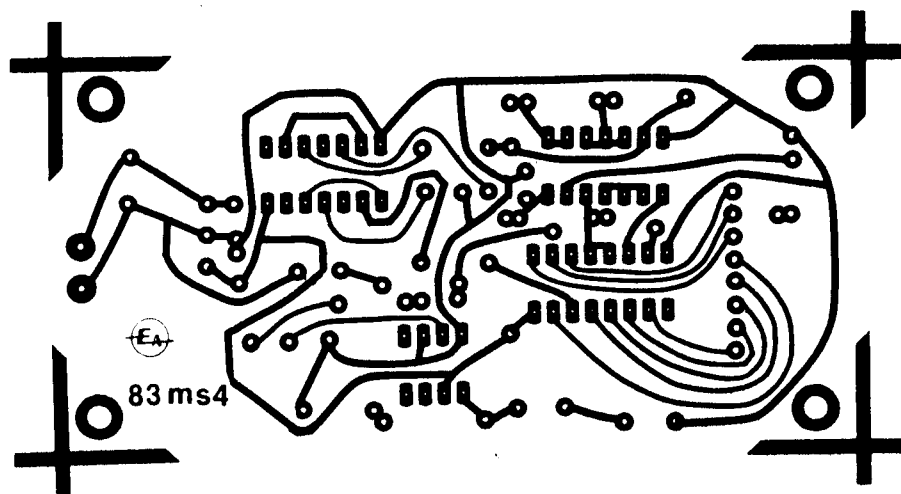
Above is the full-size pattern for the Compumuse printed circuit board.
